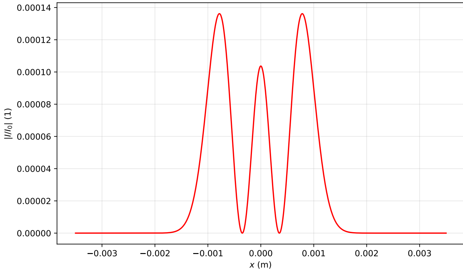
Intensity profile I(x, y = 0, z = 0.000)/I_0 , P_{in}=0.5P_{cr} , artificial time
